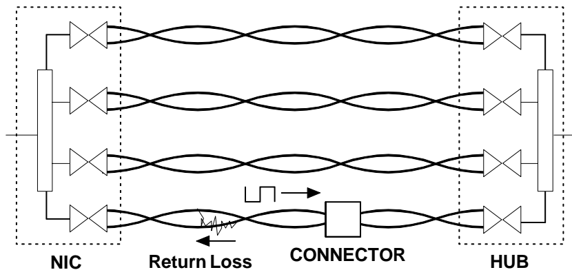
Figure 7 – Return Loss
